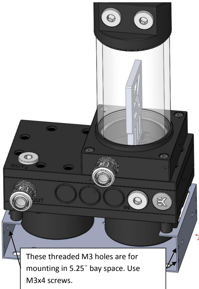
Complete assembly
