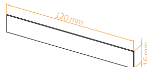
Thermal Pad F 1.0 mm (5 pcs)
