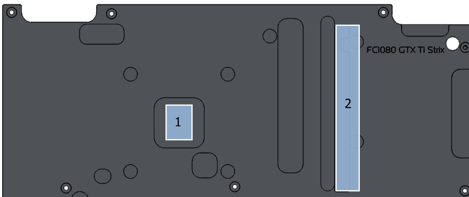
EK-FC1080 GTX Strix Backplate
