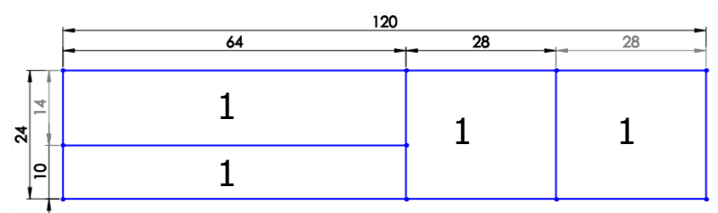
Thermal PAD G - 1mm (120x24mm)
