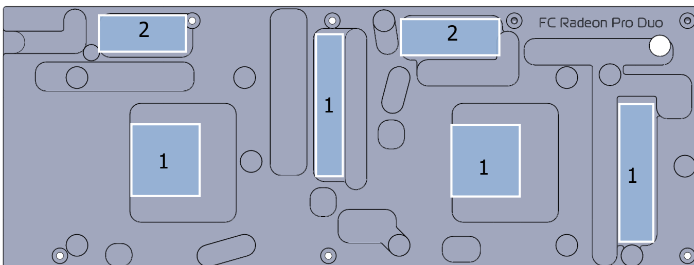
EK-FC Radeon Pro Duo Backplate
