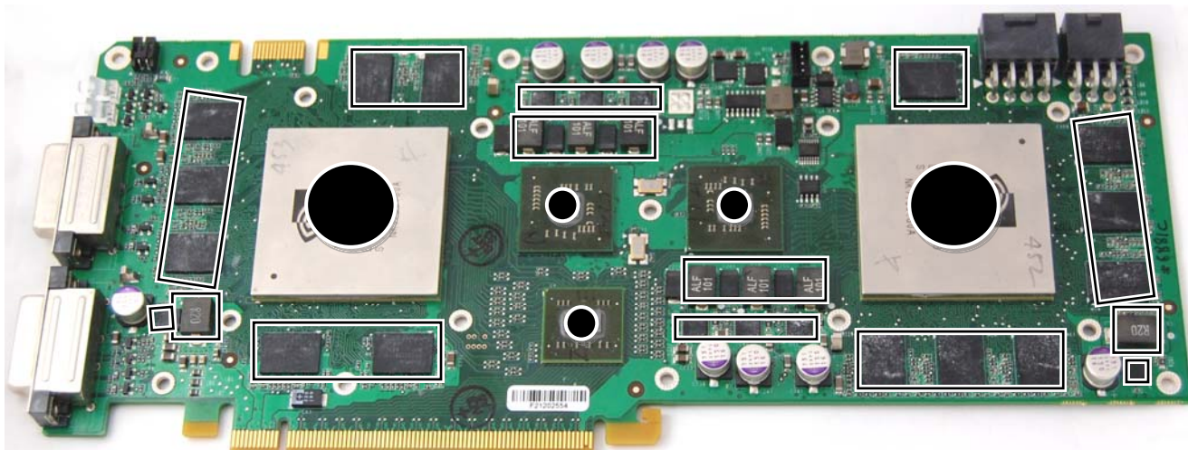
Picture 3: Applying thermal compound and thermal pads on 295GTX single PCB. Circled placed must be greased whilst squared one should be covered with thermal pads (1mm thickness). Please cut enclosed thermal pads to match needed sizes.
