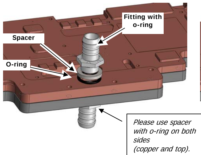
Picture 1: Sample picture of fitting installation.
