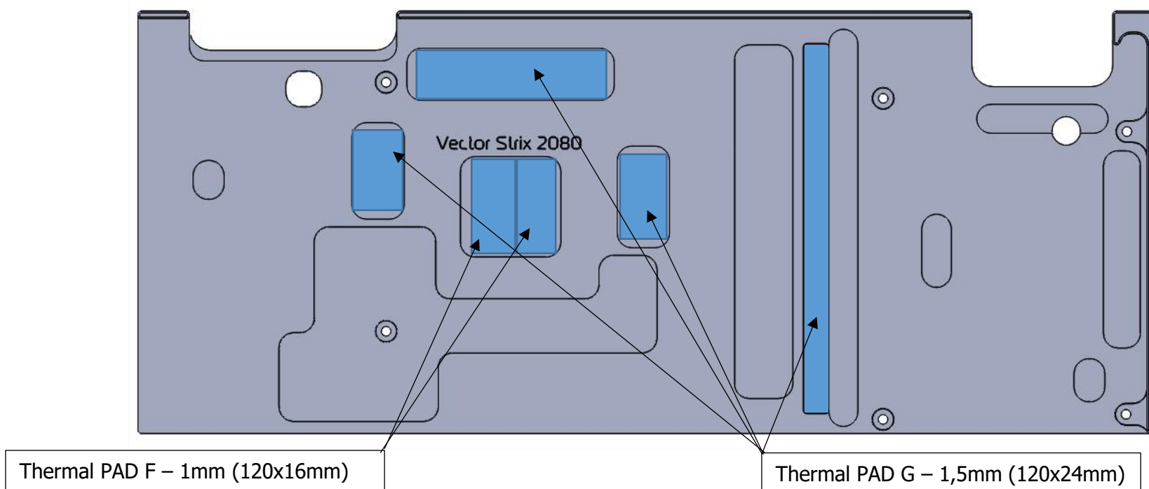
EK-Vector Strix RTX 2080 Backplate
