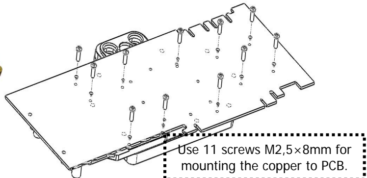
Picture 7: Mounting the water block with enclosed M2,5 screws.
