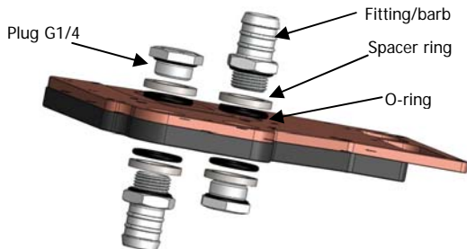
Picture 1: Spacer ring with o-ring placement.
