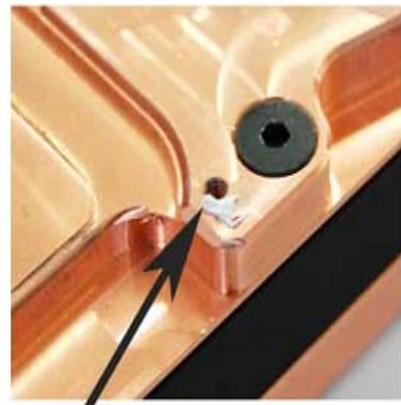
Picture 4: Apply small amount of thermal grease to fix the standoffs on right position
