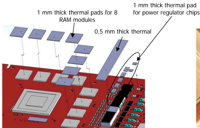
Picture 3: Radeon 4890 series graphic card. Cut thermal pads on size that fits RAM modules and VRC. Place them as shown on picture. Thermal pads are adhesive, so no extra glue is needed.
