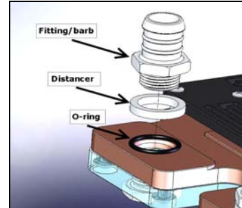
Picture 2: Distancer with o-ring placement.
