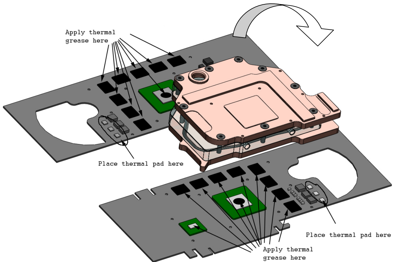
Picture 10: Applying thermal compound.
