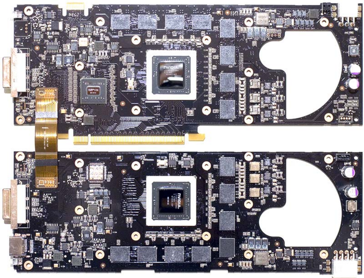
Picture 2: disassembled GeForce 9800 GX2 series graphic card without cooler.
