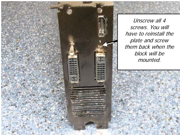
Picture 7: Disassembling the screws for VGA connectors
