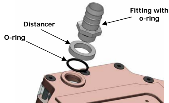
Picture 1: Fitting and plug spacer with o-ring.
