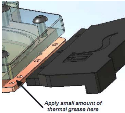
Picture 1: Installing the ALU power regulator cooler.
