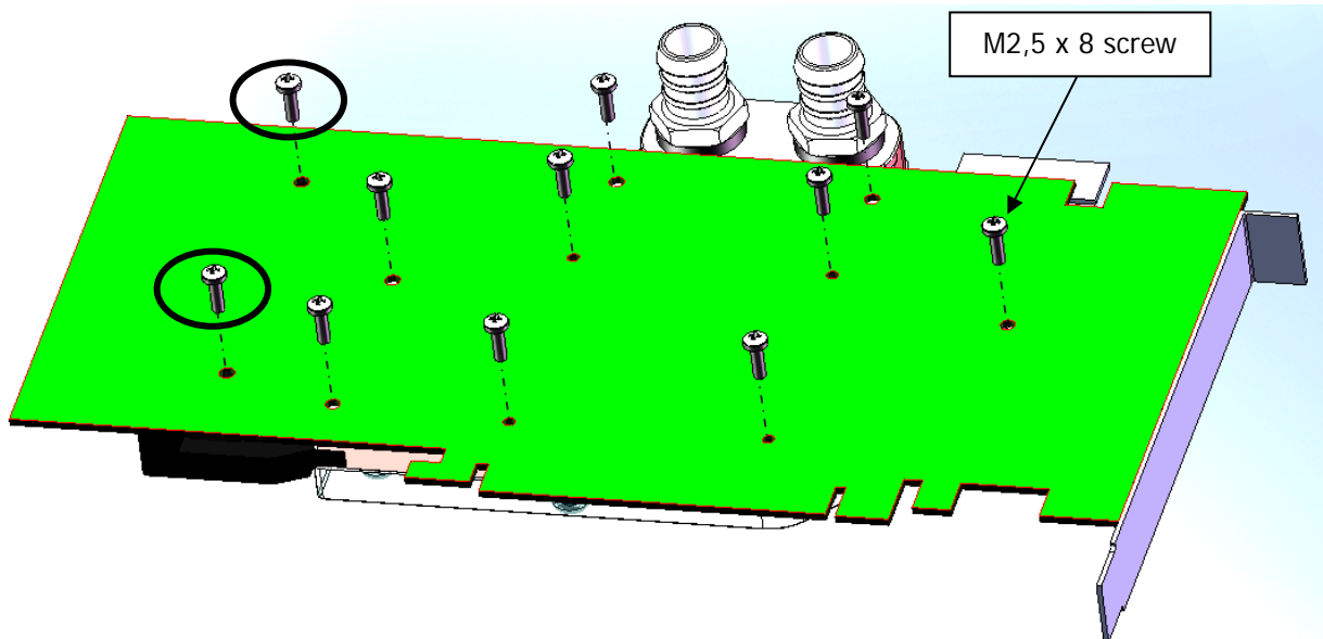
Picture 2: Mounting installation:
