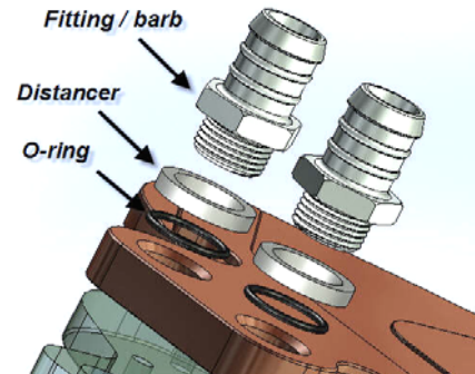
Picture 2: Distancer with o-ring placement.
