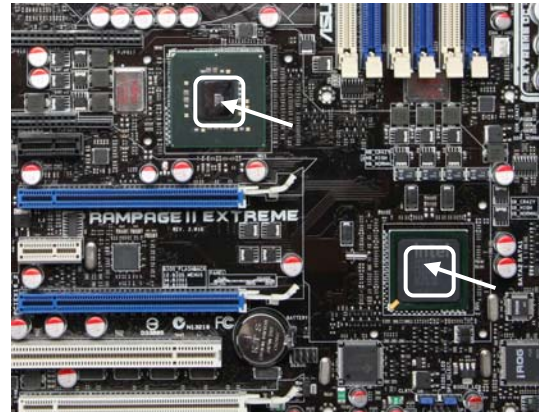
Picture 6: Apply thermal grease on NB and SB chipsets like shown in step 3.
