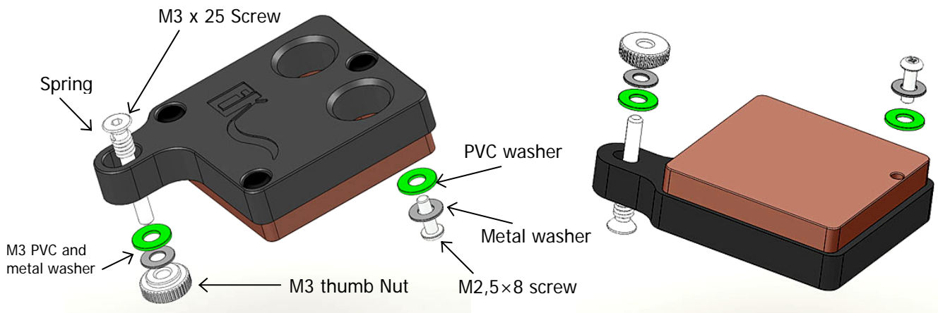
Picture 1 and 2: Installing EK-SB VGA 790i
